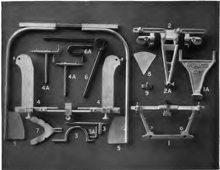
Fig. 115. The parts of the Gyst Adaptable Articulator are as follows: Nos. 1-2, upper and lower parts of articulator frame which carry the upper and lower model bows. Nos. 1A and 2A, upper and lower model bows. Nos. 3-3 Straight Incisor Guide Pin and Curved Incisor Guide Pin. The curved pin is used only when mounting models or setting anteriors. No. 3A Small pin for all set screws. Nos. 4-4 Frame work of Condyle Path Register. Nos. 4A-4A Pencil holders and pencils of Condyle Path Register. Nos. 5-5 Lateral Path Register. Nos. 6-6A Stand and gooseneck for holding Condyle Path Register and models. No. 7 Horseshoe plate. No. 8 Degree plate for measuring inclinations of paths. No. 9 Incisor Path Register.
